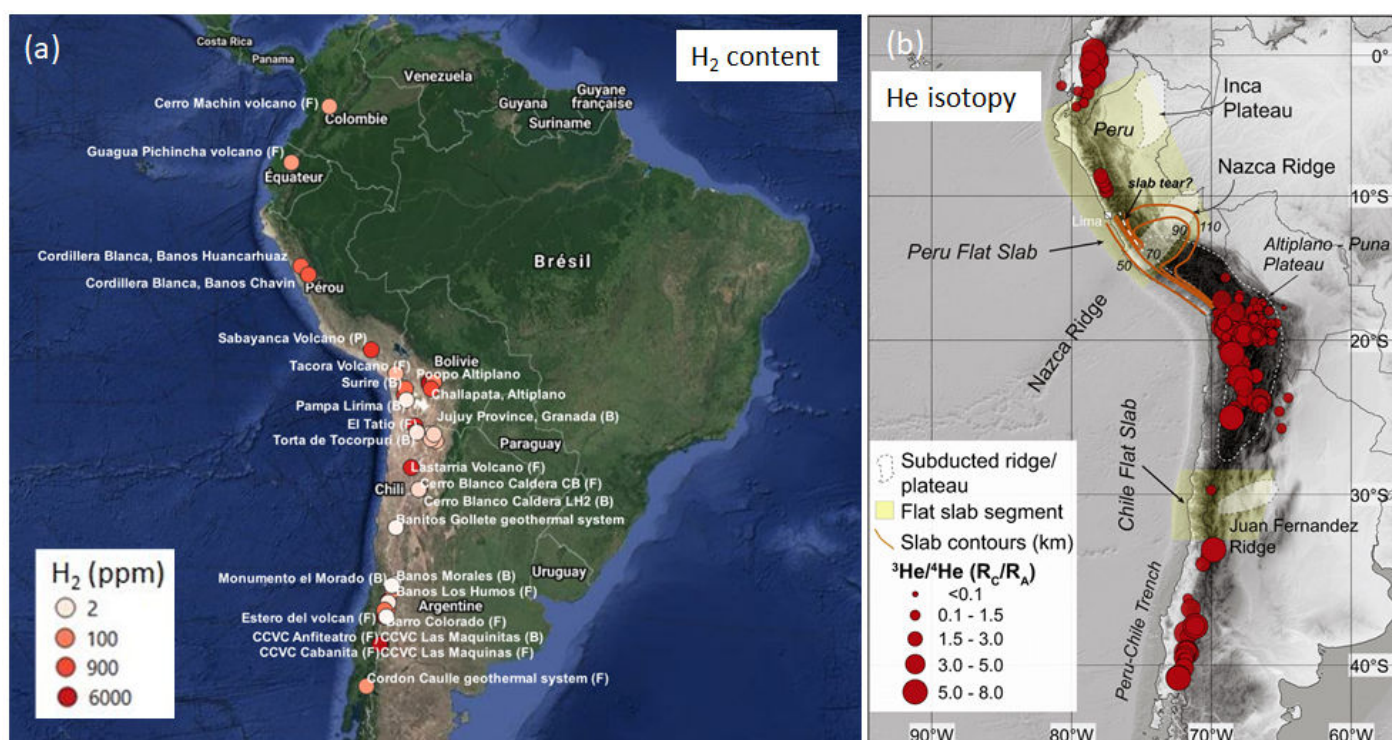
Figure 1. (a) Compilation of known \text{H}_2 leakages at the scale of the Andes. The highest values reach 5% in Chile. Co—Chanco, F—fumaroles, B—bubbling pool. (b) Helium isotopy along the Andes showing the importance of the mantellic gases and the difference between the flat slab area and the dipping slab area (modified from [17]). The highest values are between 20 and 25° S.
