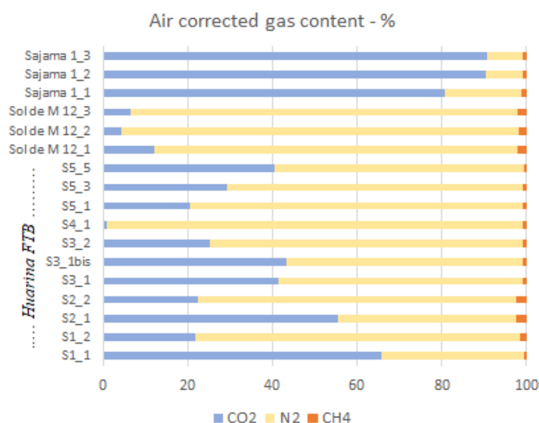
Figure 7. Main gas content after air correction. The Sol de Mañana area is characterized by its N 2 content (>85%), and the Sajama area is characterized by its CO 2 content (>80%). On the eastern border faults, it is a blend.
